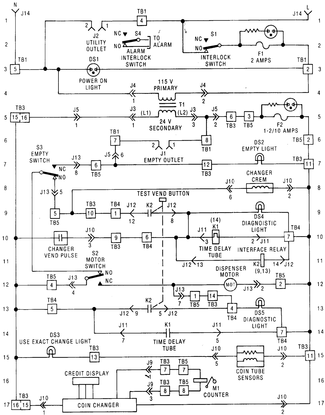
PBM-4 SCHEMATIC DIAGRAM
