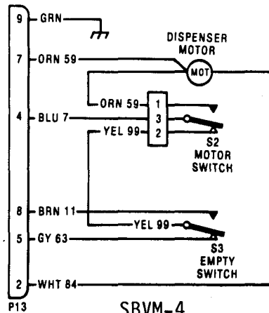
SBVM-4 Dispenser Diagram 1237035
