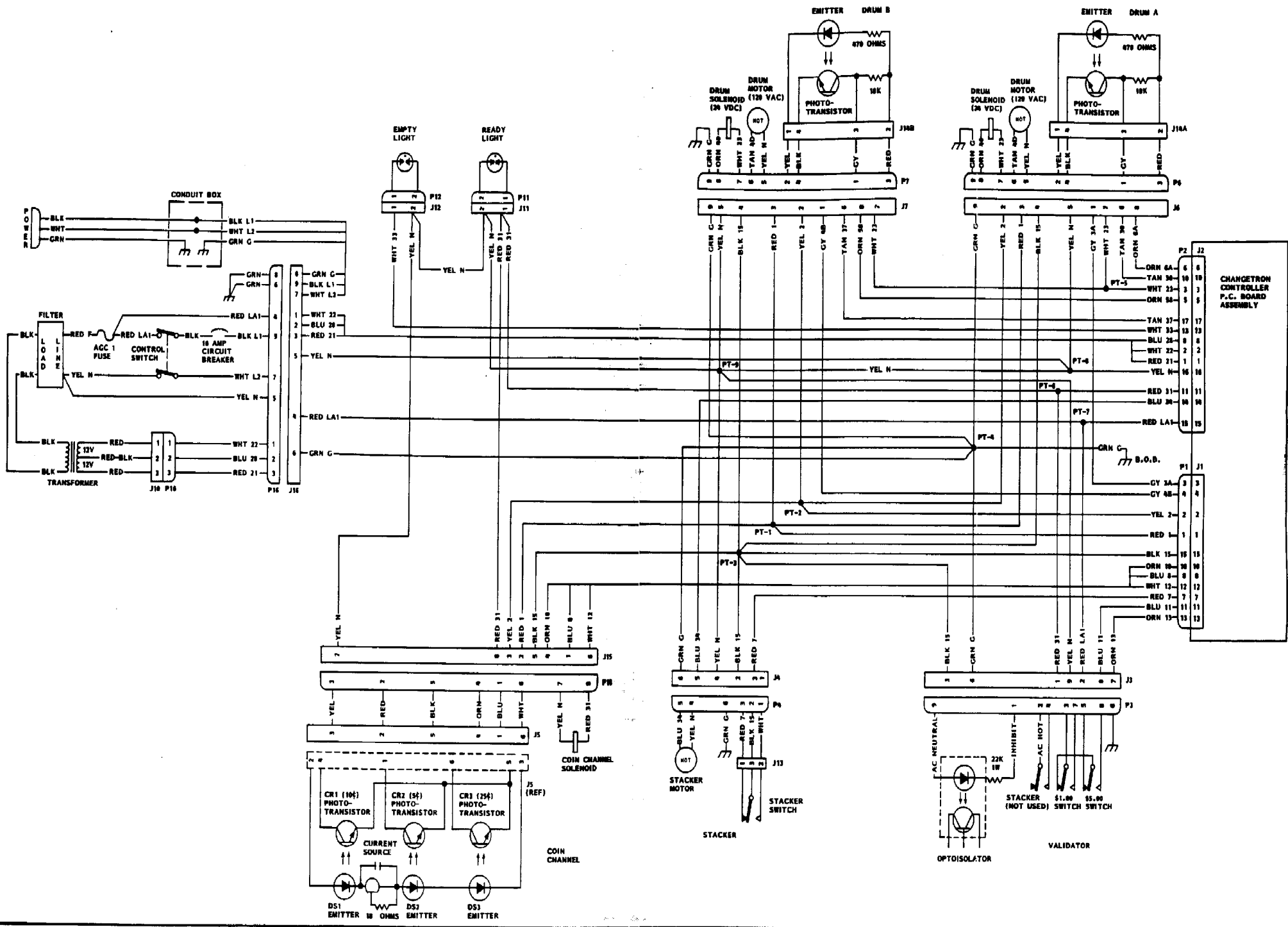
Figure 5-1, Changetron 2 Wiring Diagram
