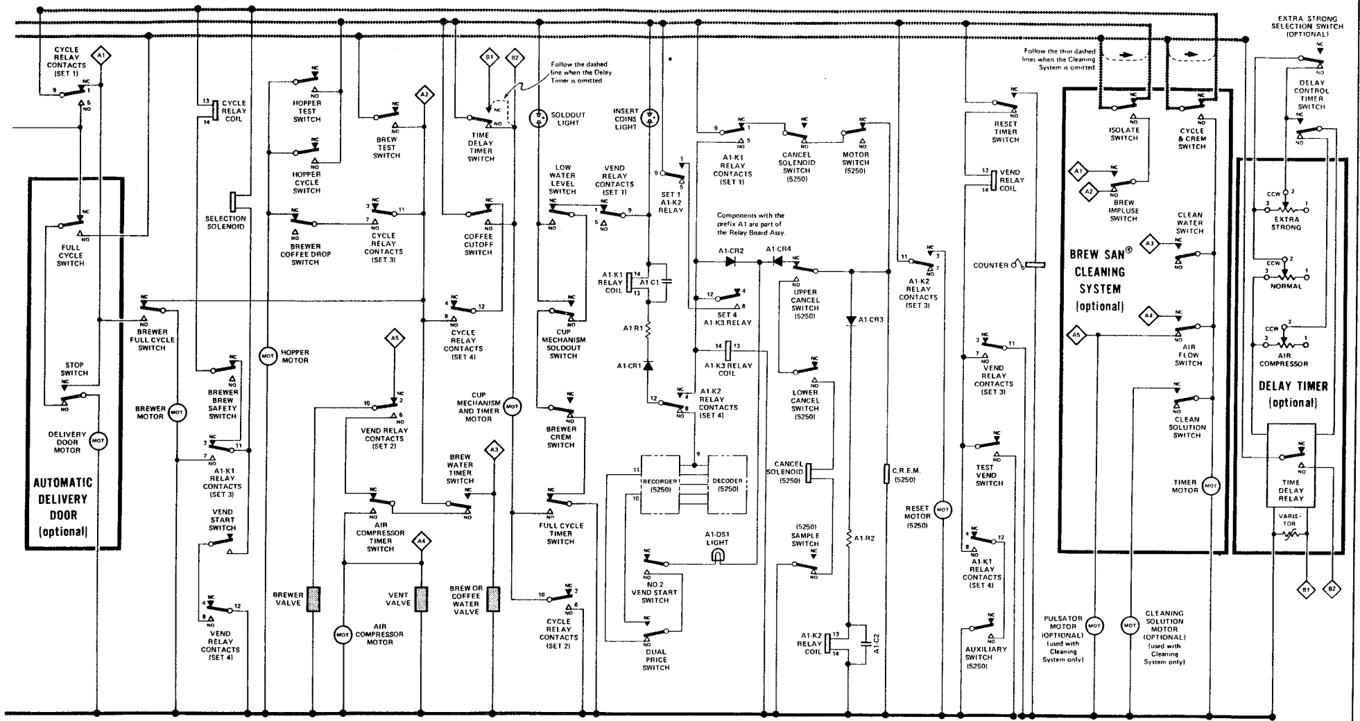
Figure 6-4. The Merchandiser Schematic Diagram with 5250 ACER (2 of 2)
